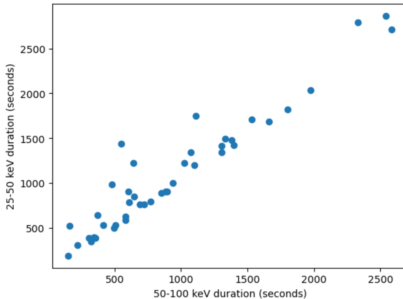
25-50 keV duration vs 50-100 keV duration
